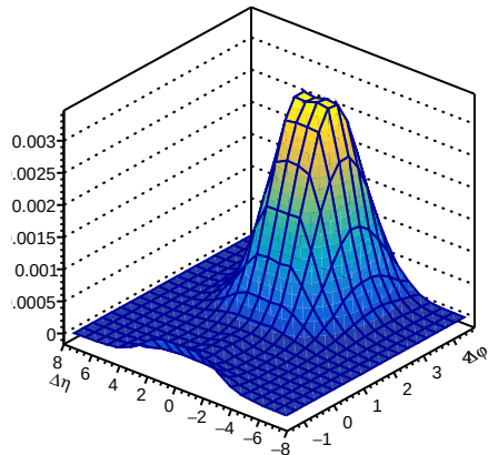
D^+D^- OS - SS, 20-60%, per trigger
