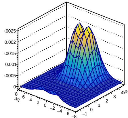
D^+D^- OS - SS, 60-100%, per trigger
