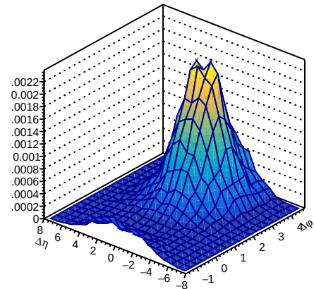
B^+B^- OS - SS, 60-100%, per trigger
