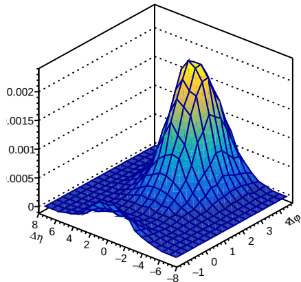
B^+B^- OS - SS, 20-60%, per trigger
