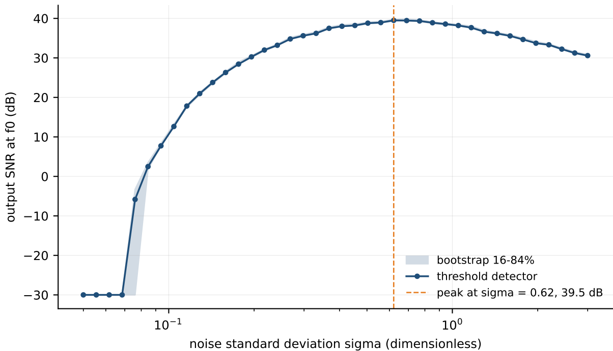
E2: threshold detector, A = 0.7 below \theta = 1.0 , 20 trials
