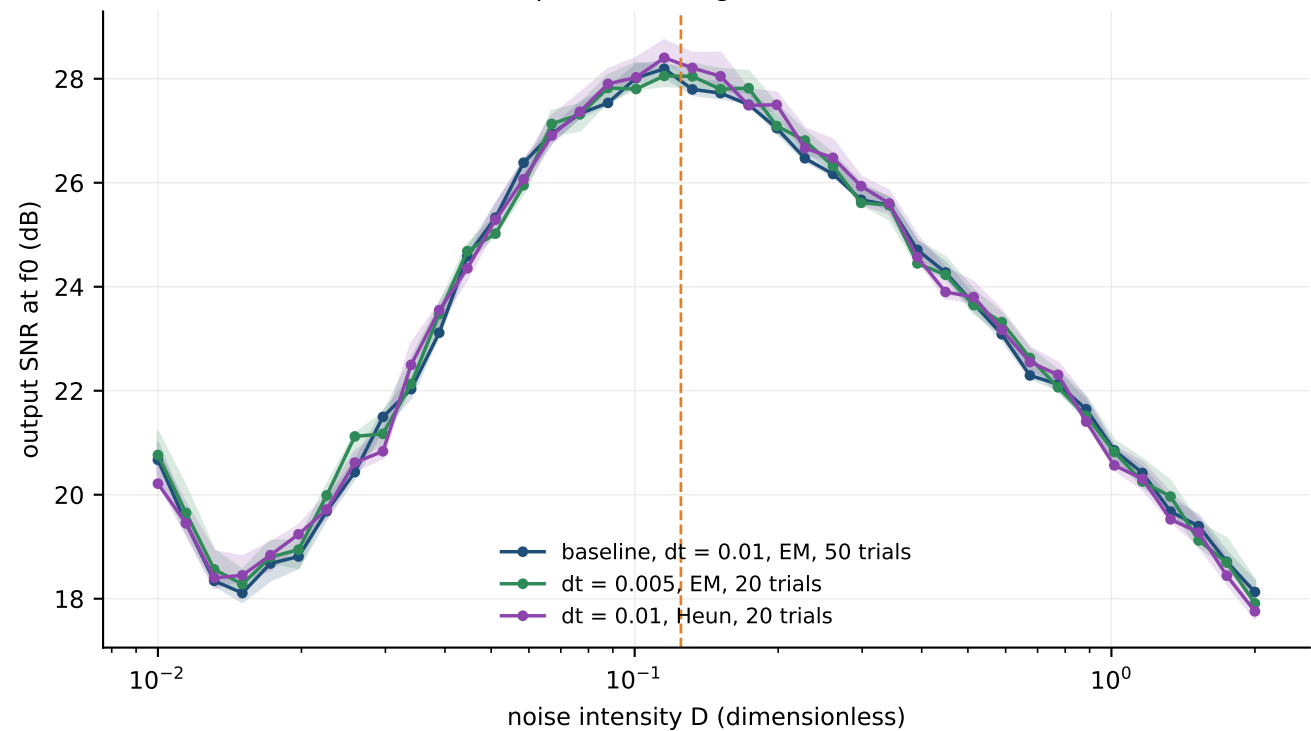
E3 numerical checks: halved step and Heun against the baseline
