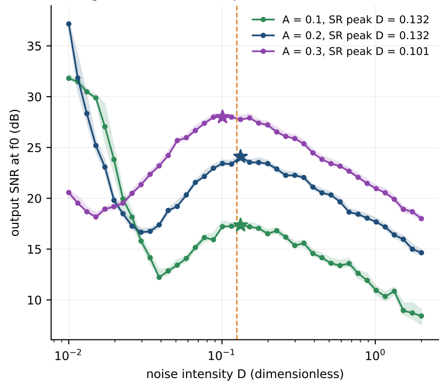
SNR against D for three amplitudes, f_0 = 0.01
