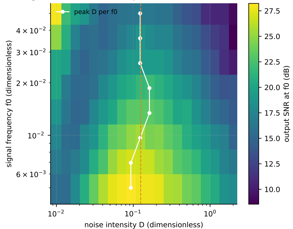
SNR over (D, f_0) , 64 periods, 10 trials
