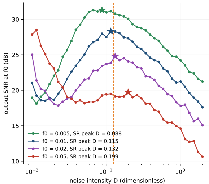
SNR against D for four frequencies (bandwidth differs, see docstring)
