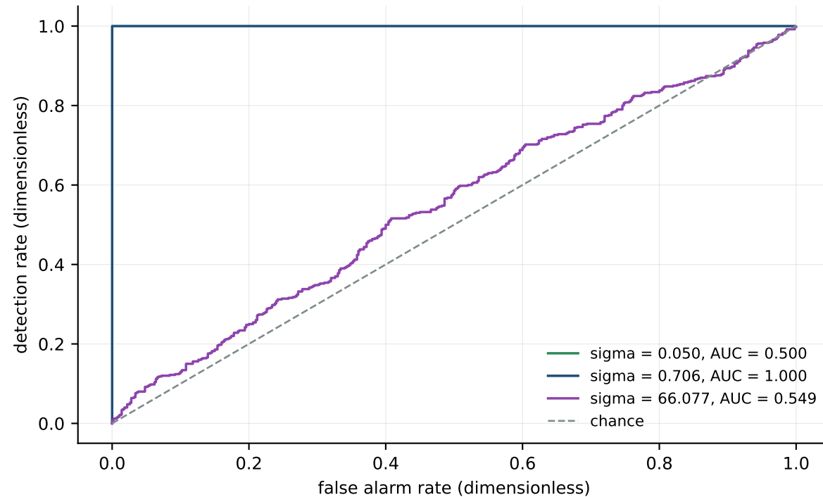
Threshold detector, A = 0.7 : ROC at three sigma
