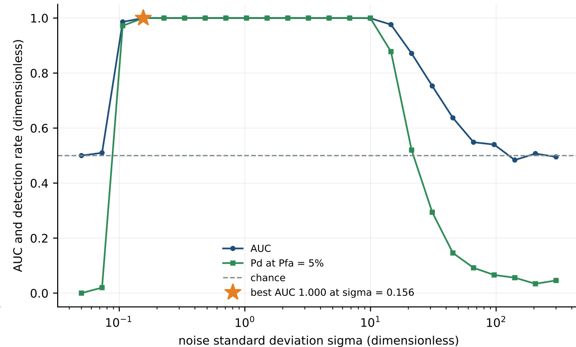
Threshold detector: noise does help detection
