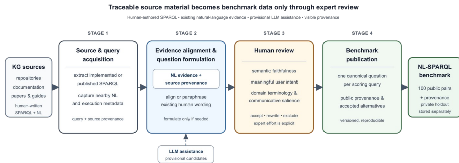
Fig. 1. Musparql workflow. Source evidence, model proposals, execution observations, and reviewer decisions remain separate but linked.
