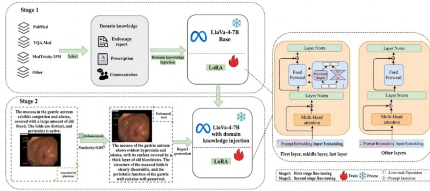
Figure 4.1: Overall architecture of the proposed two-phase fine-tuning pipeline. The left portion depicts Phases 1 (public-dataset domain injection) and 2 (private clinical fine-tuning); the right portion provides a detailed view of the P-LoRA adaptation module. Green-highlighted components indicate the elements introduced in this work.
