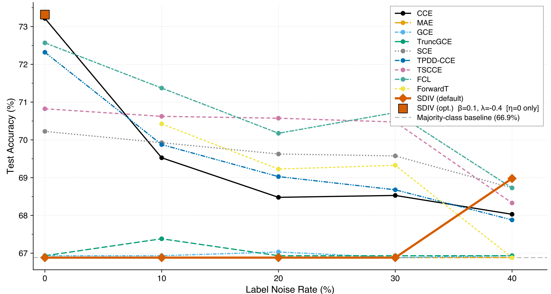
DermaMNIST: Test Accuracy under Label Noise Corruption Vision Transformer (ViT-Tiny), 7-class dermatoscopy
