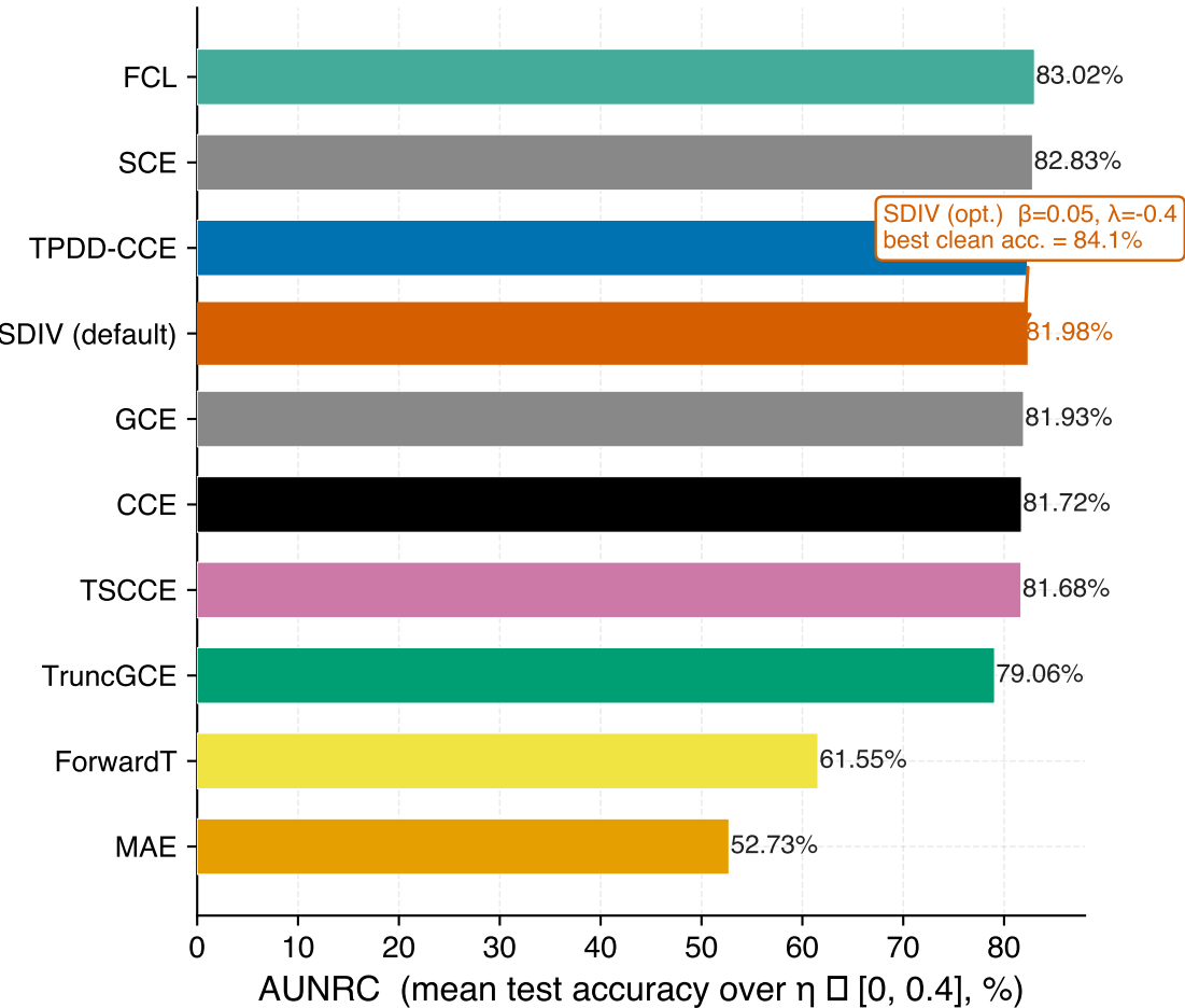
PathMNIST (9-class histopathology)
