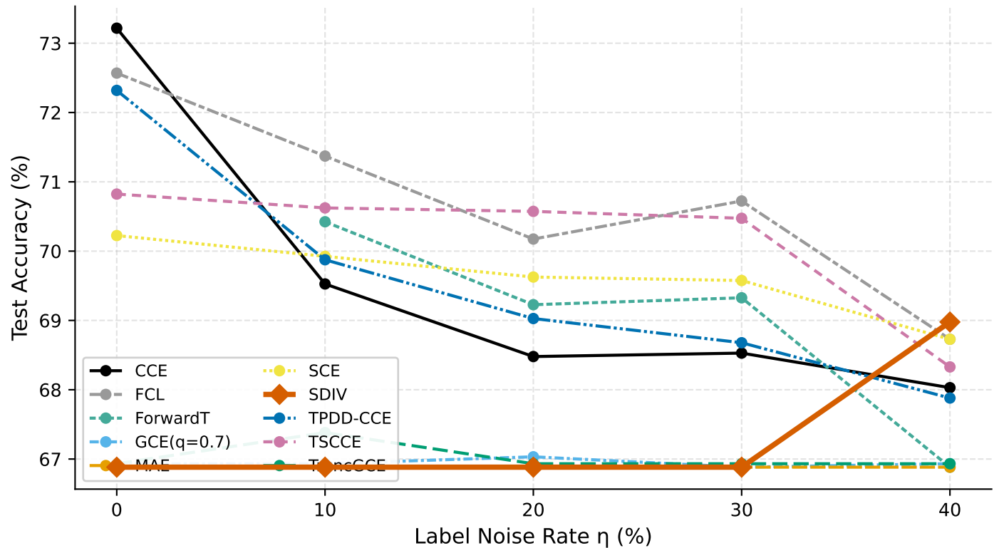
DermaMNIST: Label Noise Robustness (ViT, seed=42)
