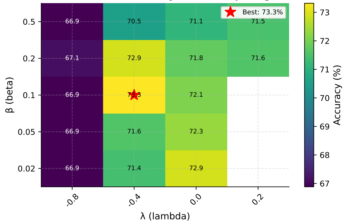
DermaMNIST: Accuracy (%) over ( \beta , \lambda ) grid
