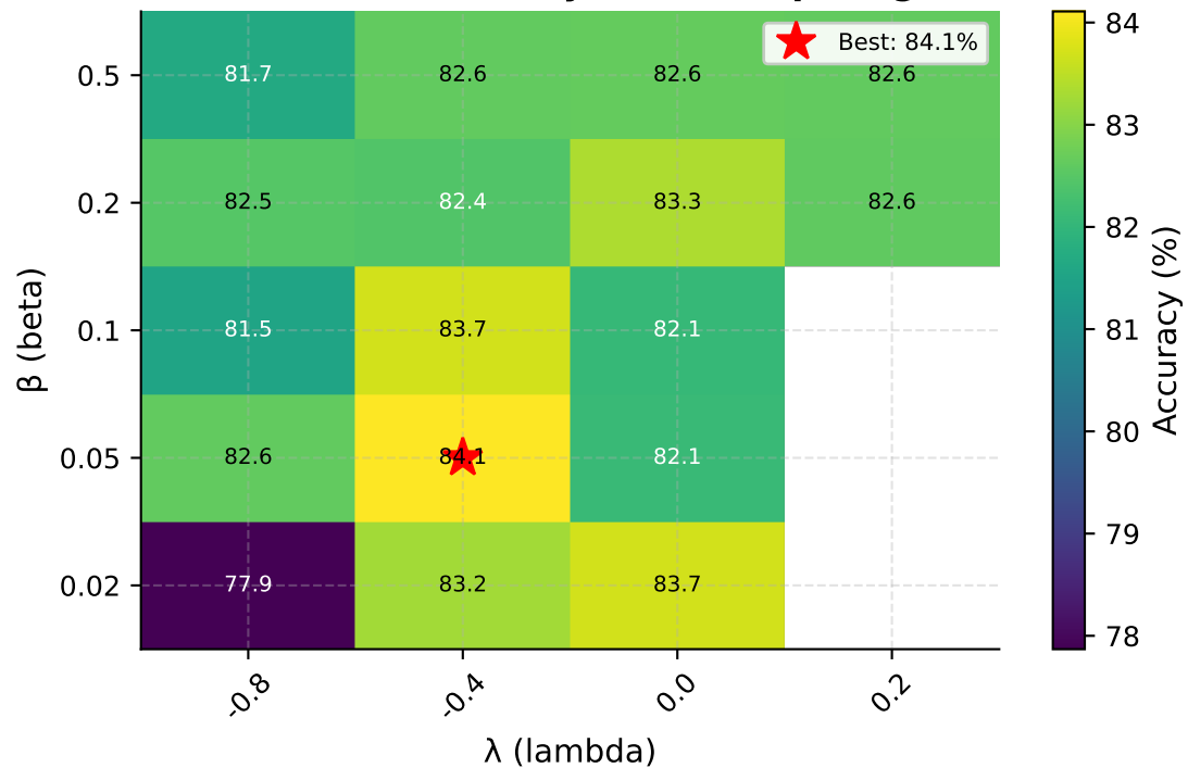
PathMNIST: Accuracy (%) over ( \beta , \lambda ) grid
