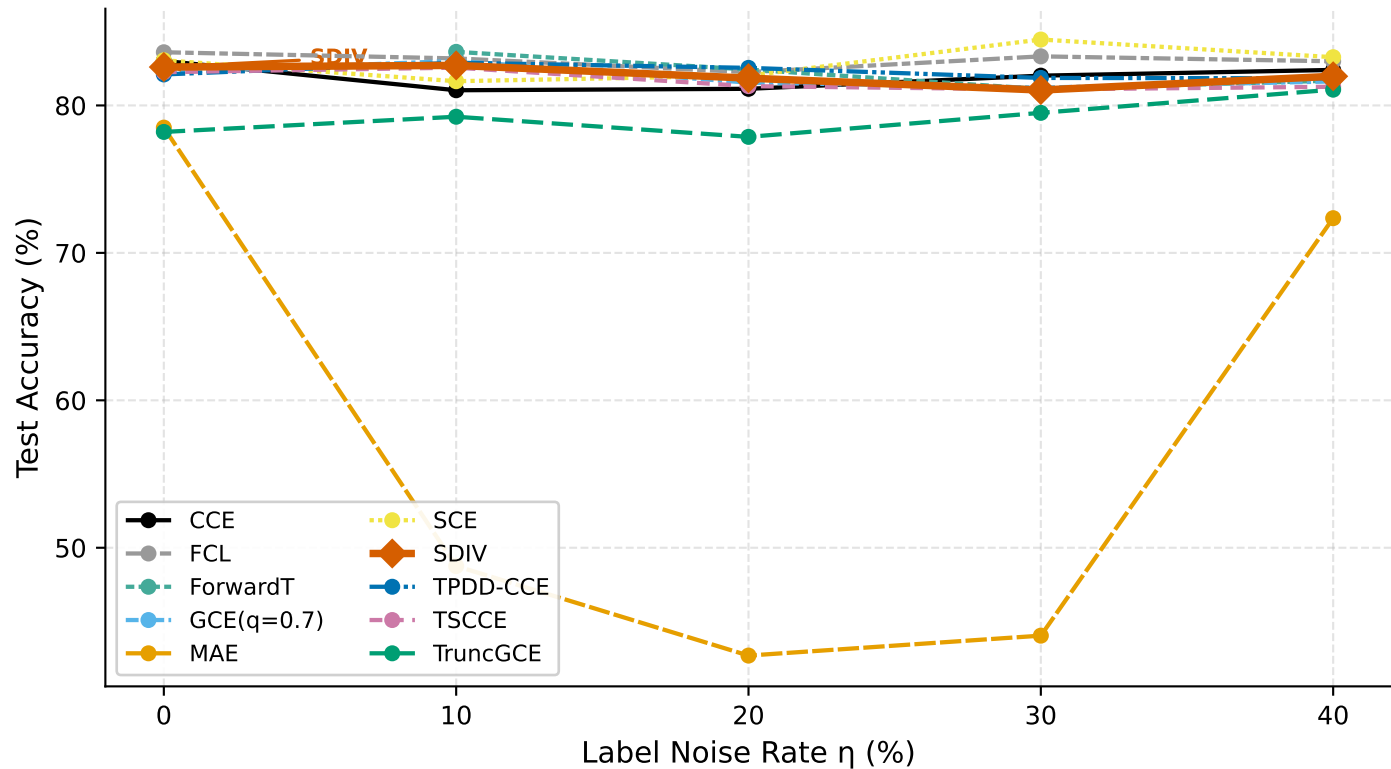
PathMNIST: Label Noise Robustness (ViT, seed=42)
