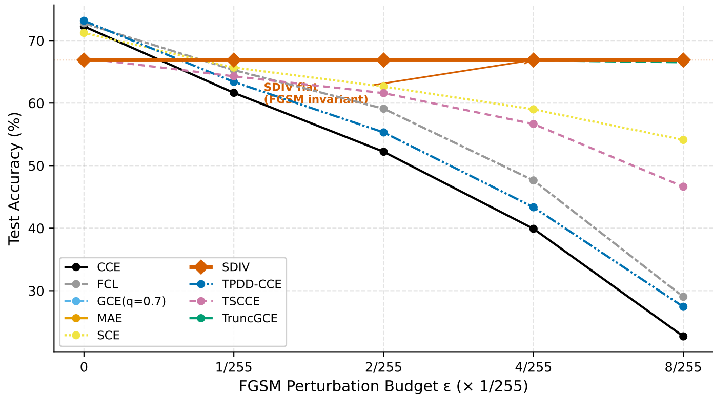
DermaMNIST: FGSM Adversarial Robustness (ViT, seed=42)
