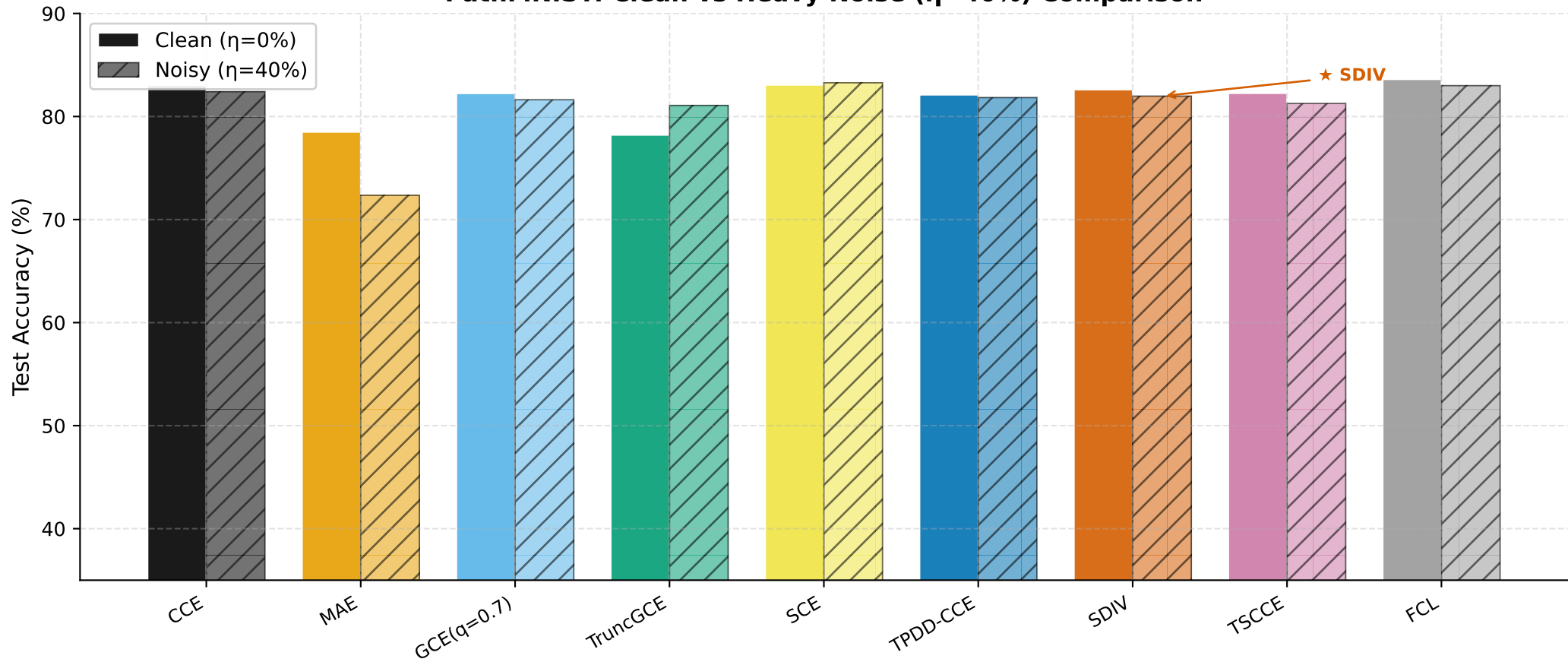
PathMNIST: Clean vs Heavy Noise ( \eta=40\% ) Comparison
