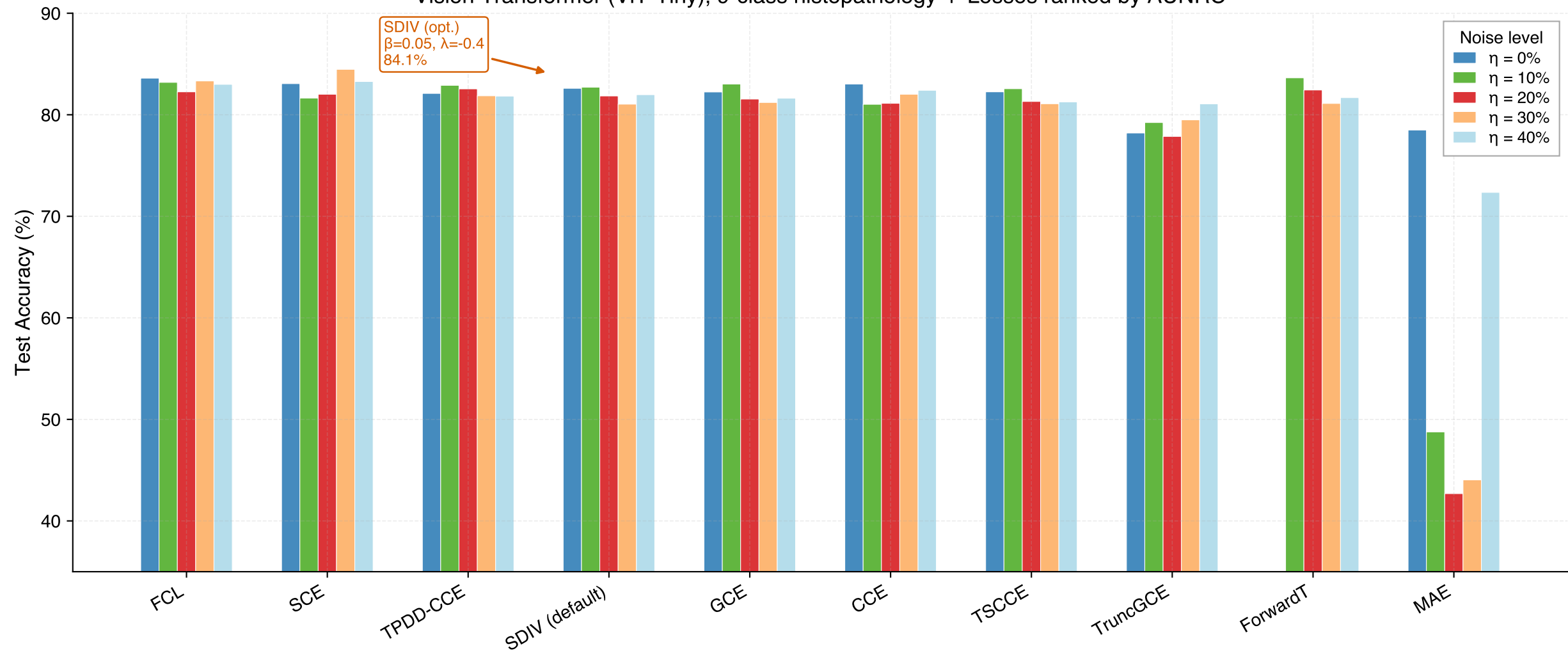
PathMNIST: Test Accuracy across Label Noise Rates Vision Transformer (ViT-Tiny), 9-class histopathology | Losses ranked by AUNRC
