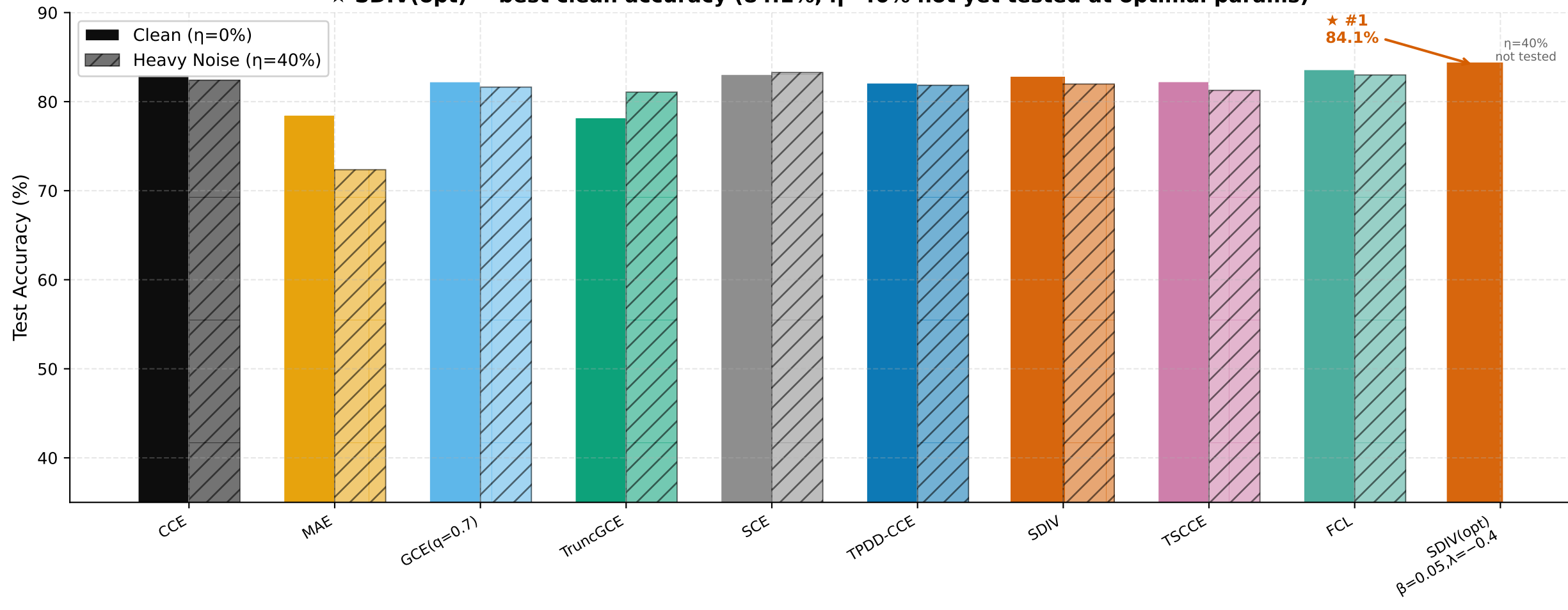
PathMNIST: Clean vs Heavy Noise ( \eta=40\% ) (seed=42, single run) ★ SDIV(opt) = best clean accuracy (84.1%, \eta=40\% not yet tested at optimal params)
