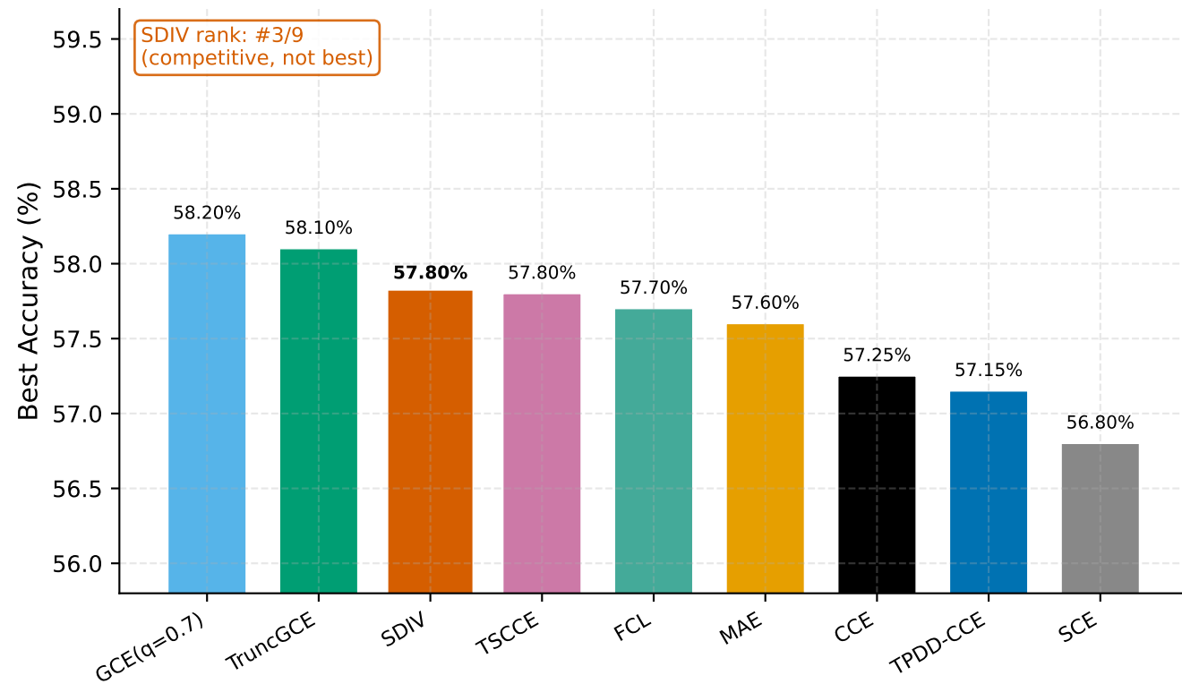
BERT on Emotion (6-class NLP)
