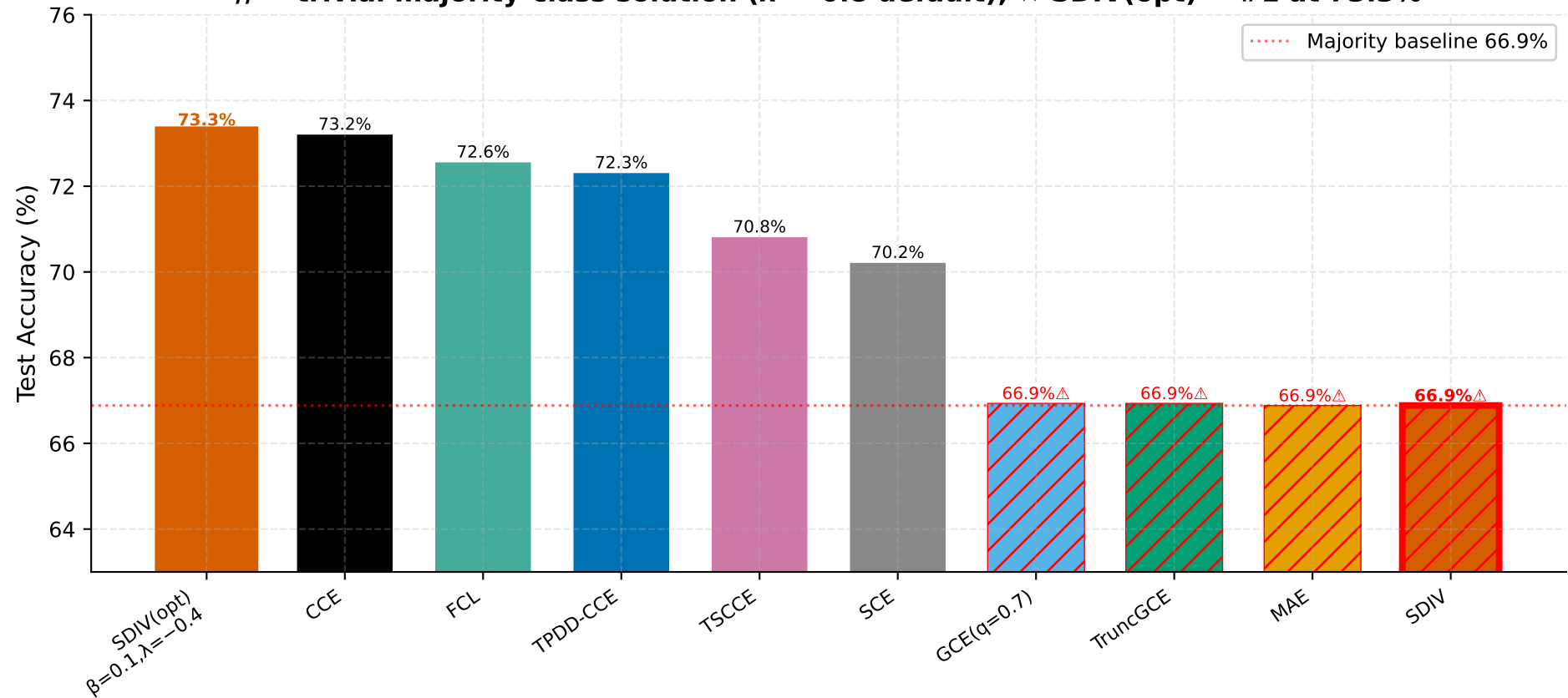
DermaMNIST Clean Accuracy ( \eta=0\% ) — All Losses (seed=42, single run) // = trivial majority-class solution ( \lambda=-0.8 default); ★ SDIV(opt) = #1 at 73.3%
