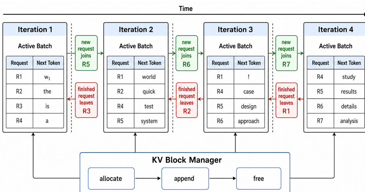
图 14 Continuous Batching / Iteration-level Batching 机制示意图
