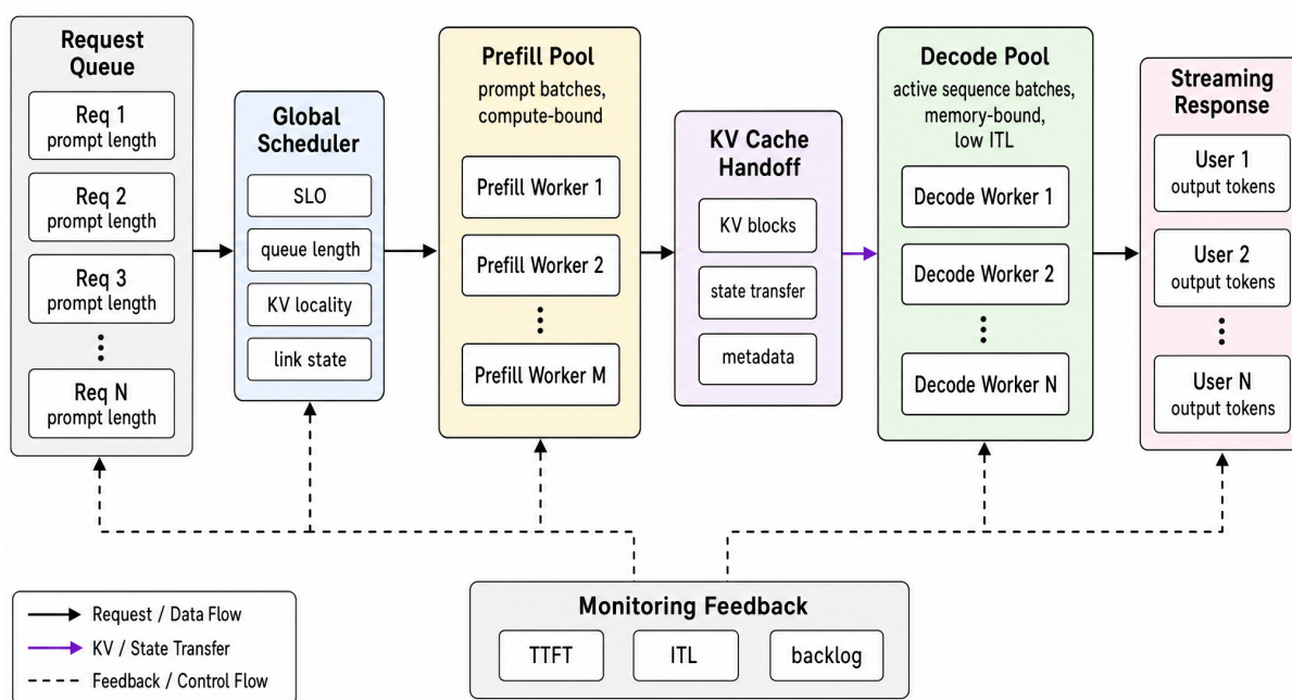
图 16 Disaggregated Prefill-Decode Batching 机制示意图
