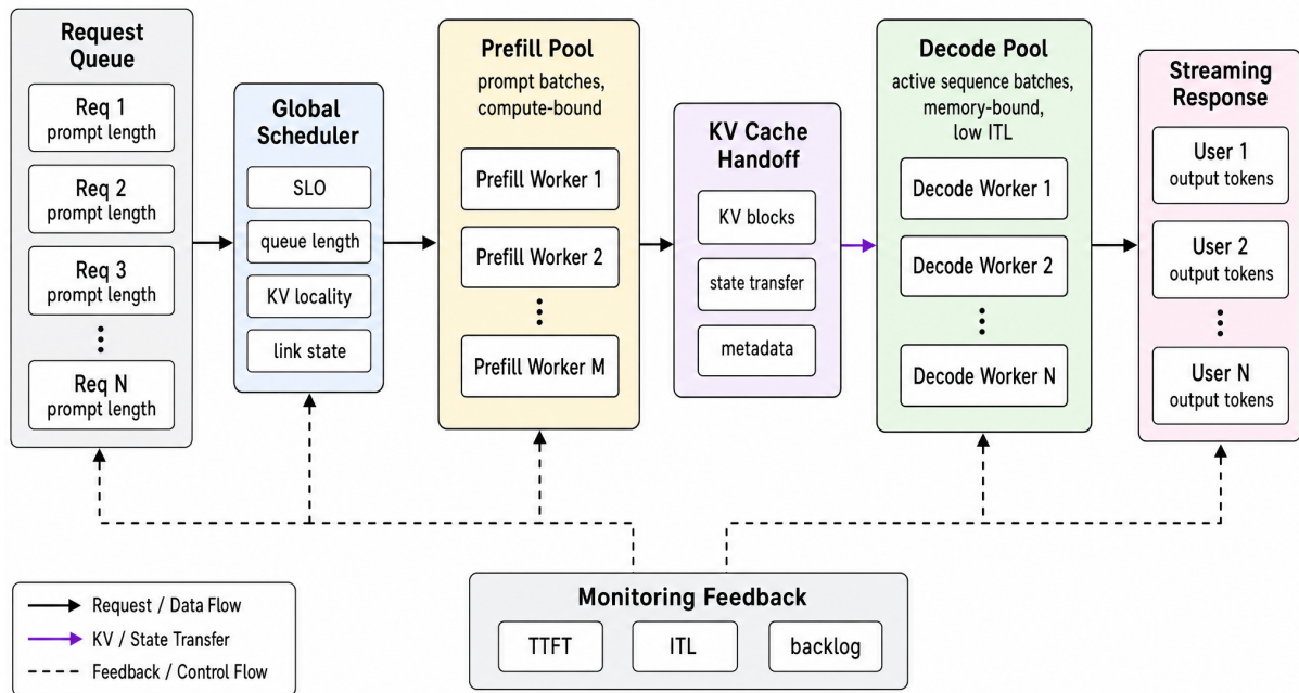
图 16 Disaggregated Prefill-Decode Batching 机制示意图
