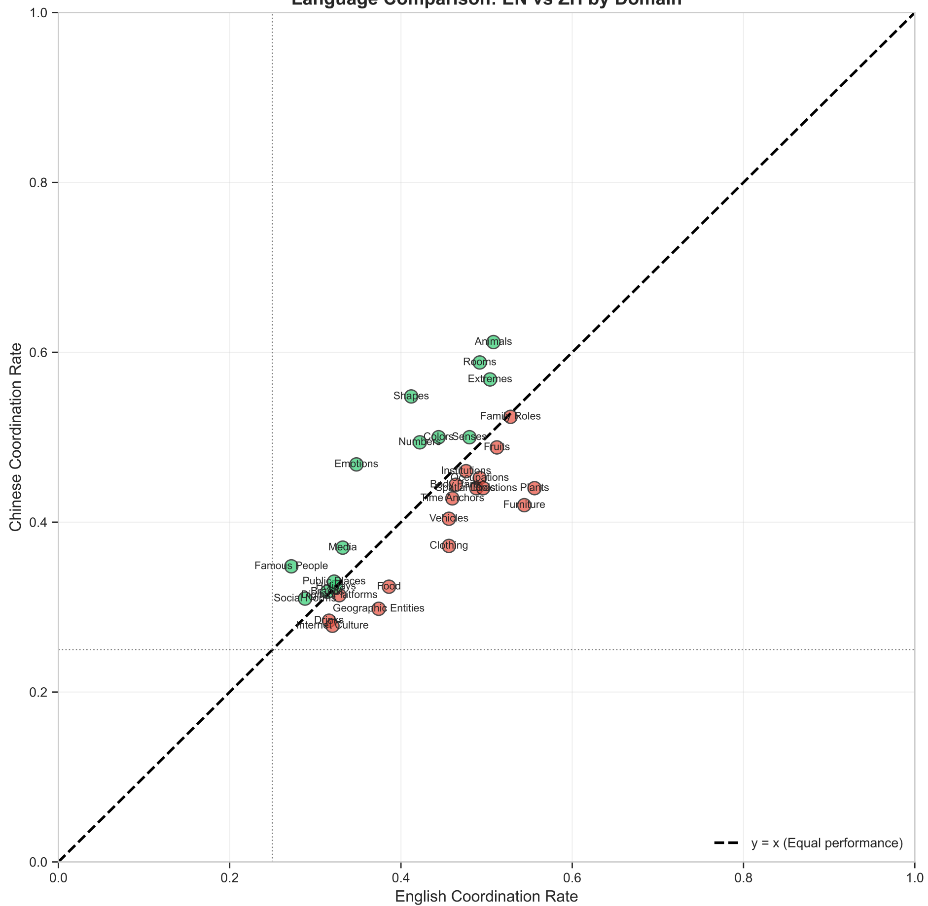
Language Comparison: EN vs ZH by Domain
