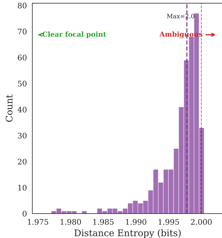
(a) Distance Entropy Distribution
