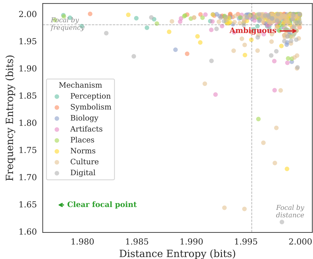
(c) 2D Item Landscape
