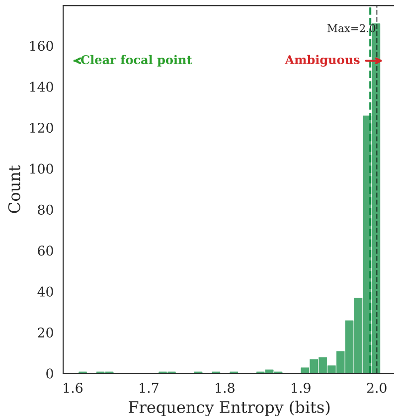
(b) Frequency Entropy Distribution
