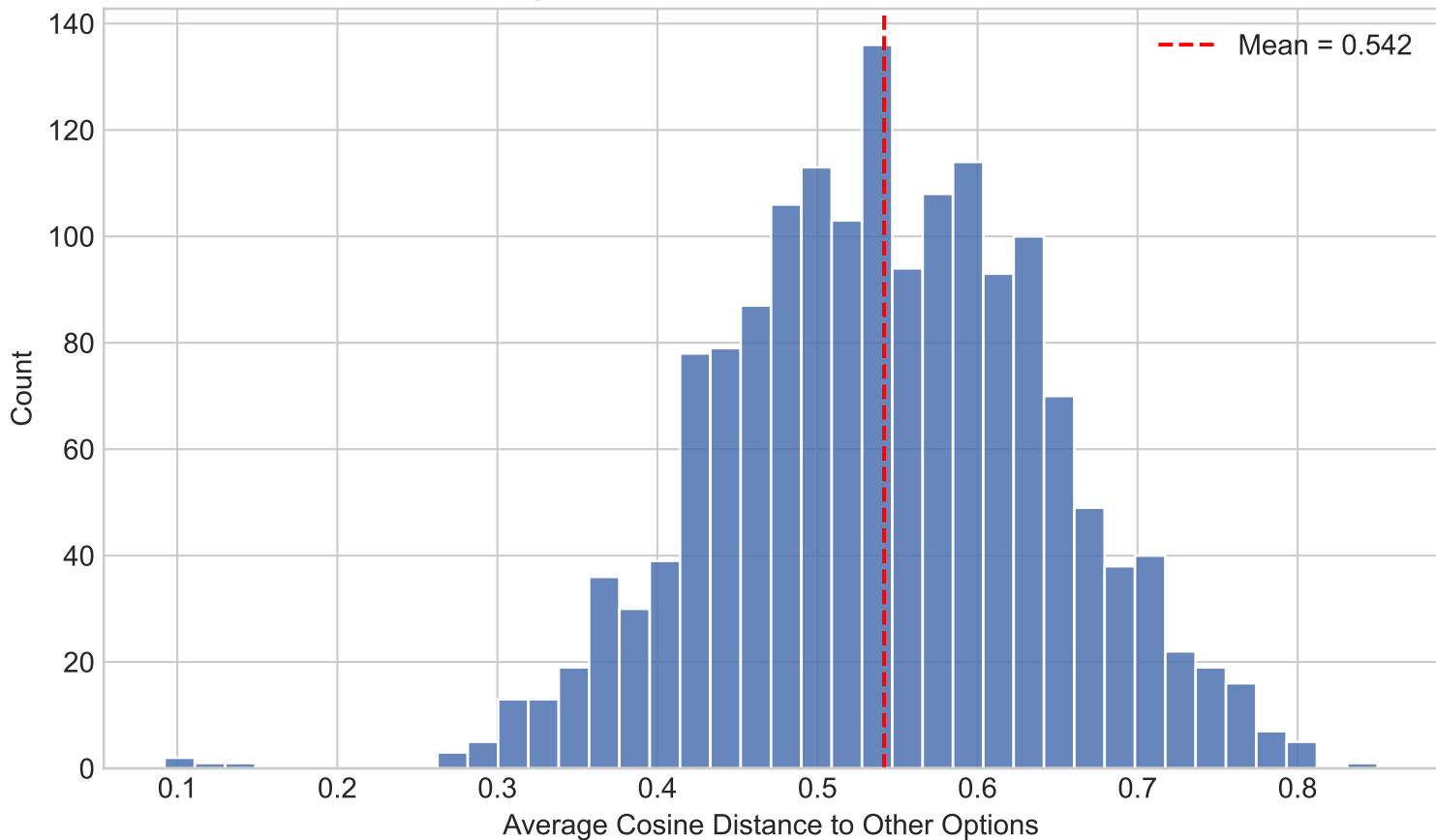
Item Quality: Distribution of Option Semantic Distance
