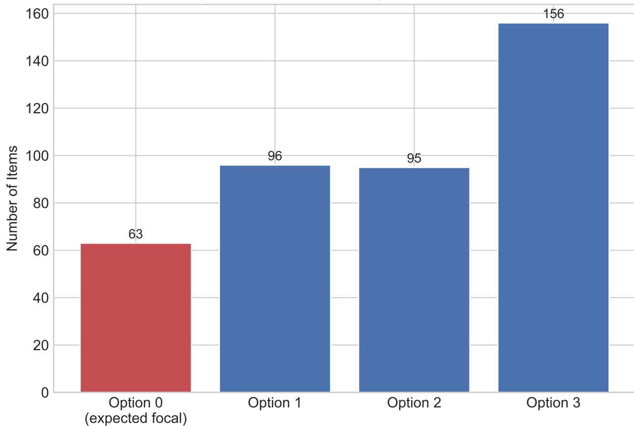
Item Quality: Which Option Has Highest Semantic Distance?
