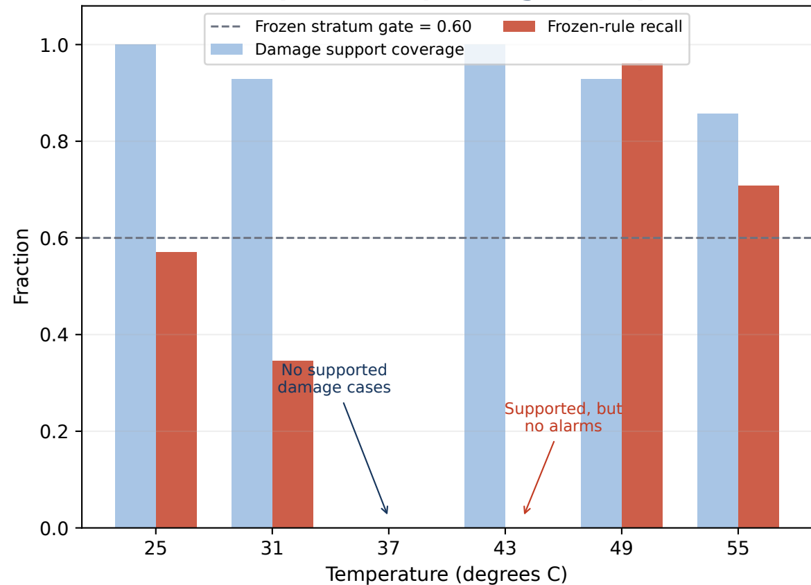
Temperature operating envelope
