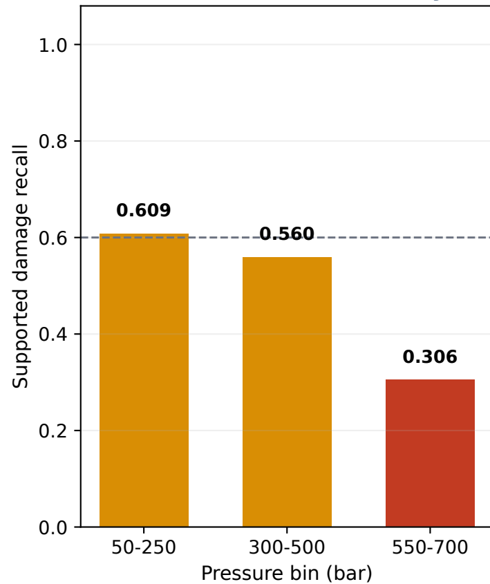
Pressure-bin sensitivity
