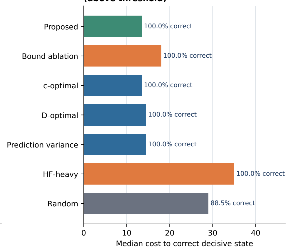
(c) True contrast \Delta = 5 (above threshold)
