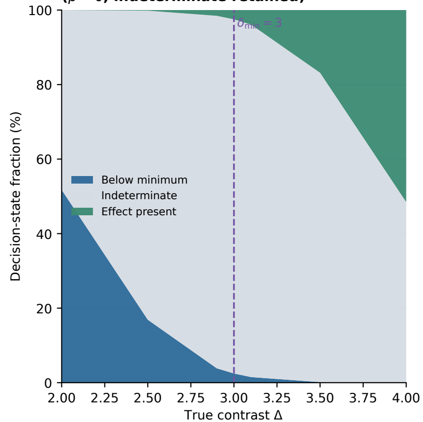
(a) Central two-sided 95% interval ( \rho = 0 ; indeterminate retained)
