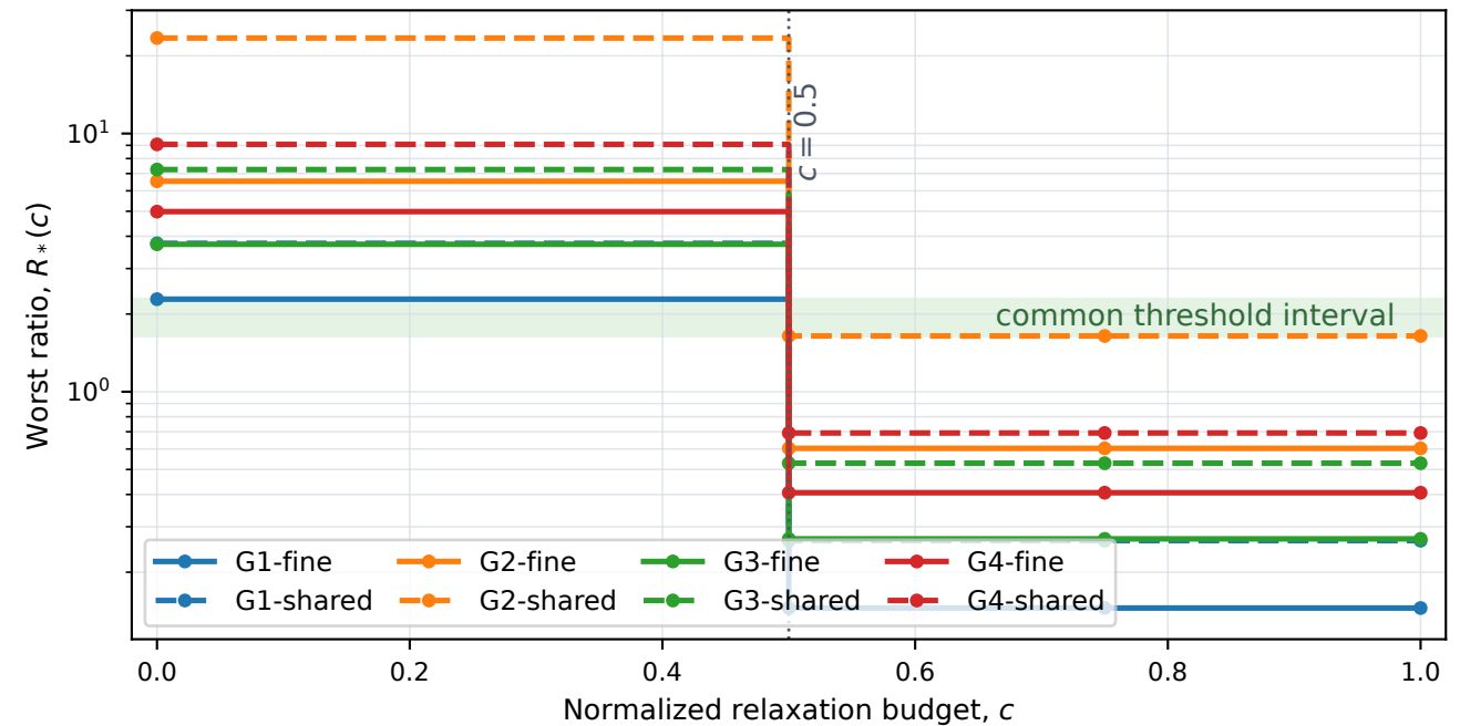
(c) Exact equality is less stable than near-attainment
