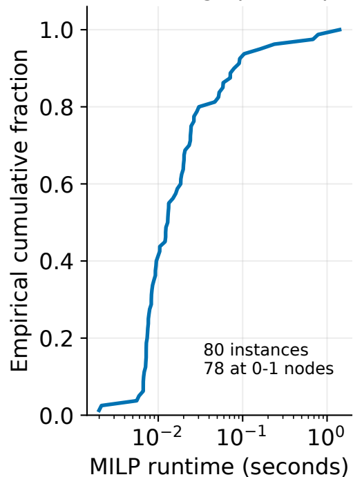
(c) General-graph test pool
