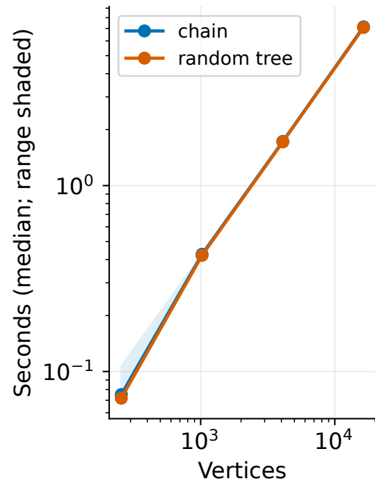
(a) Forest runtime
