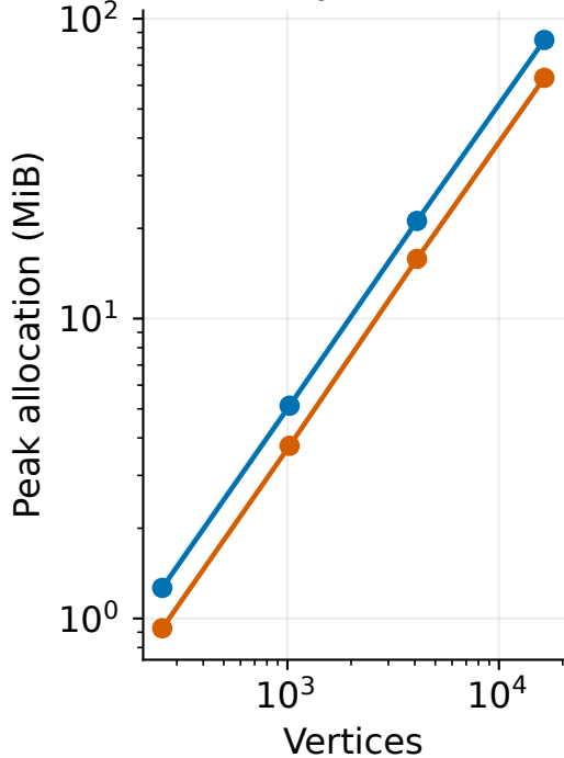
(b) Traced Python allocation
