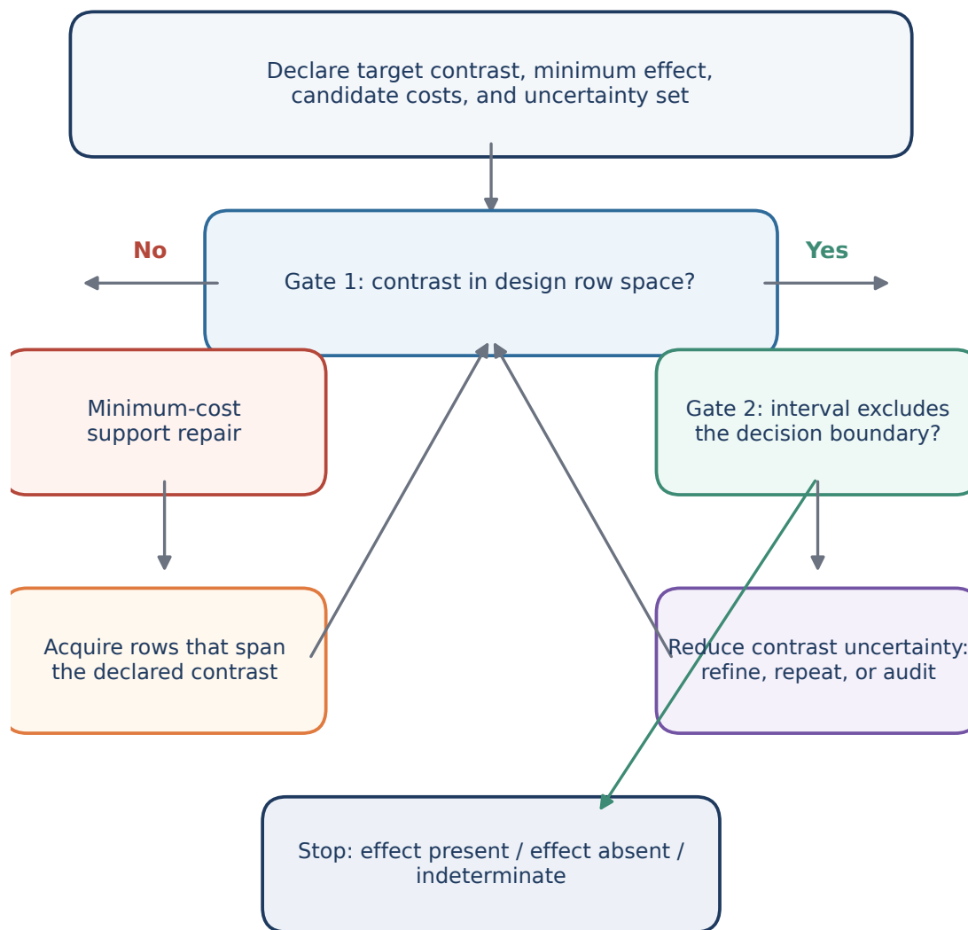
(a) Claim-adaptive decision loop
