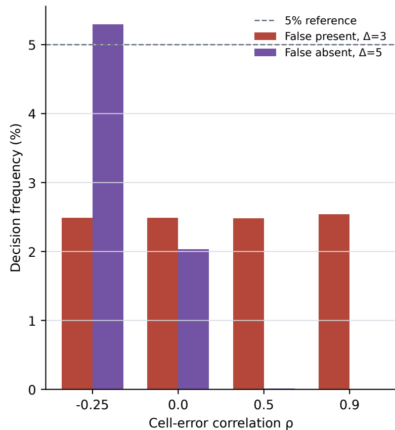
(a) Covariance-rule calibration
