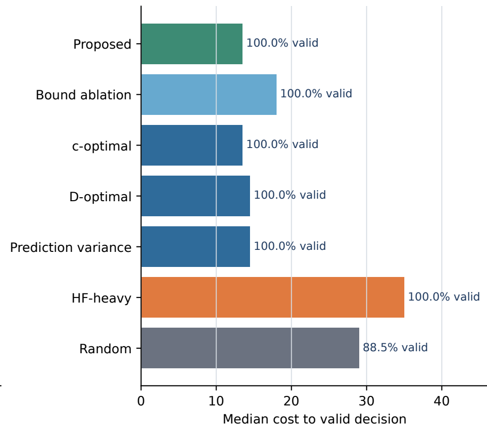
(c) True contrast \Delta=5
