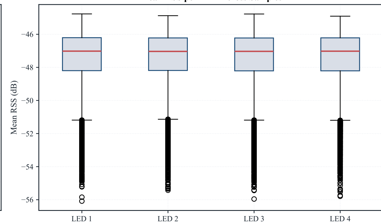
Mean RSS per LED Across Samples
