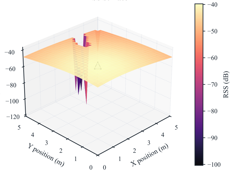
LED 3 RSS Surface
