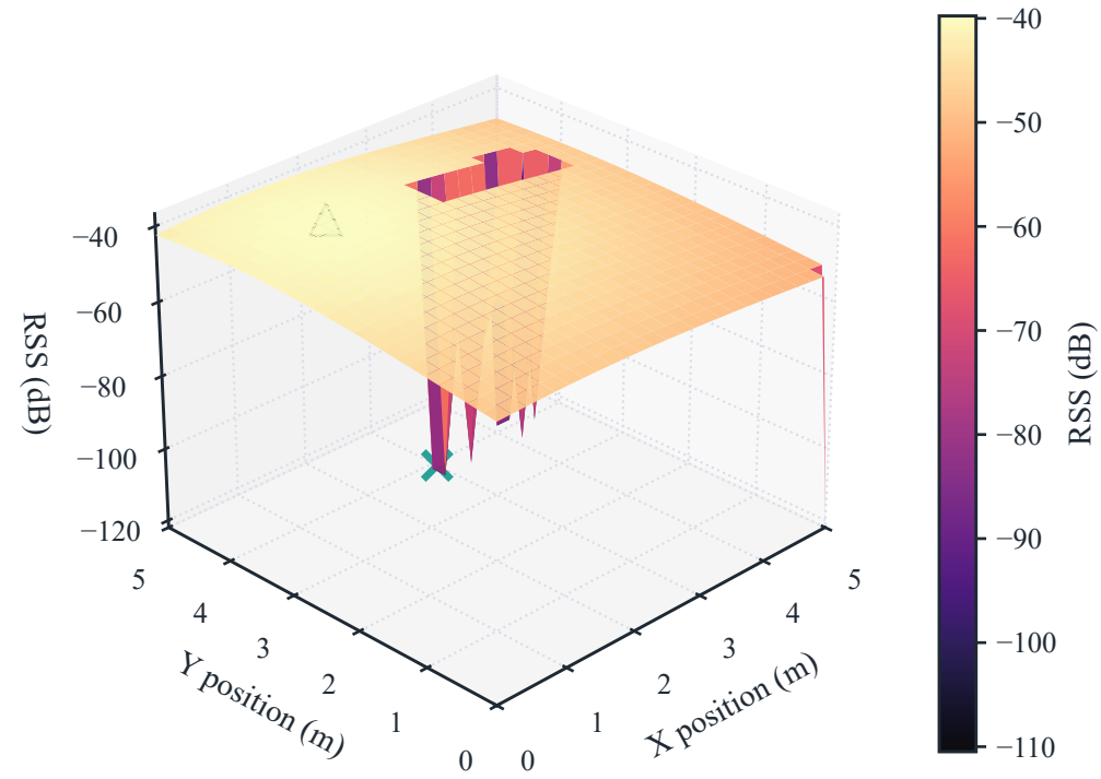
LED 4 RSS Surface
