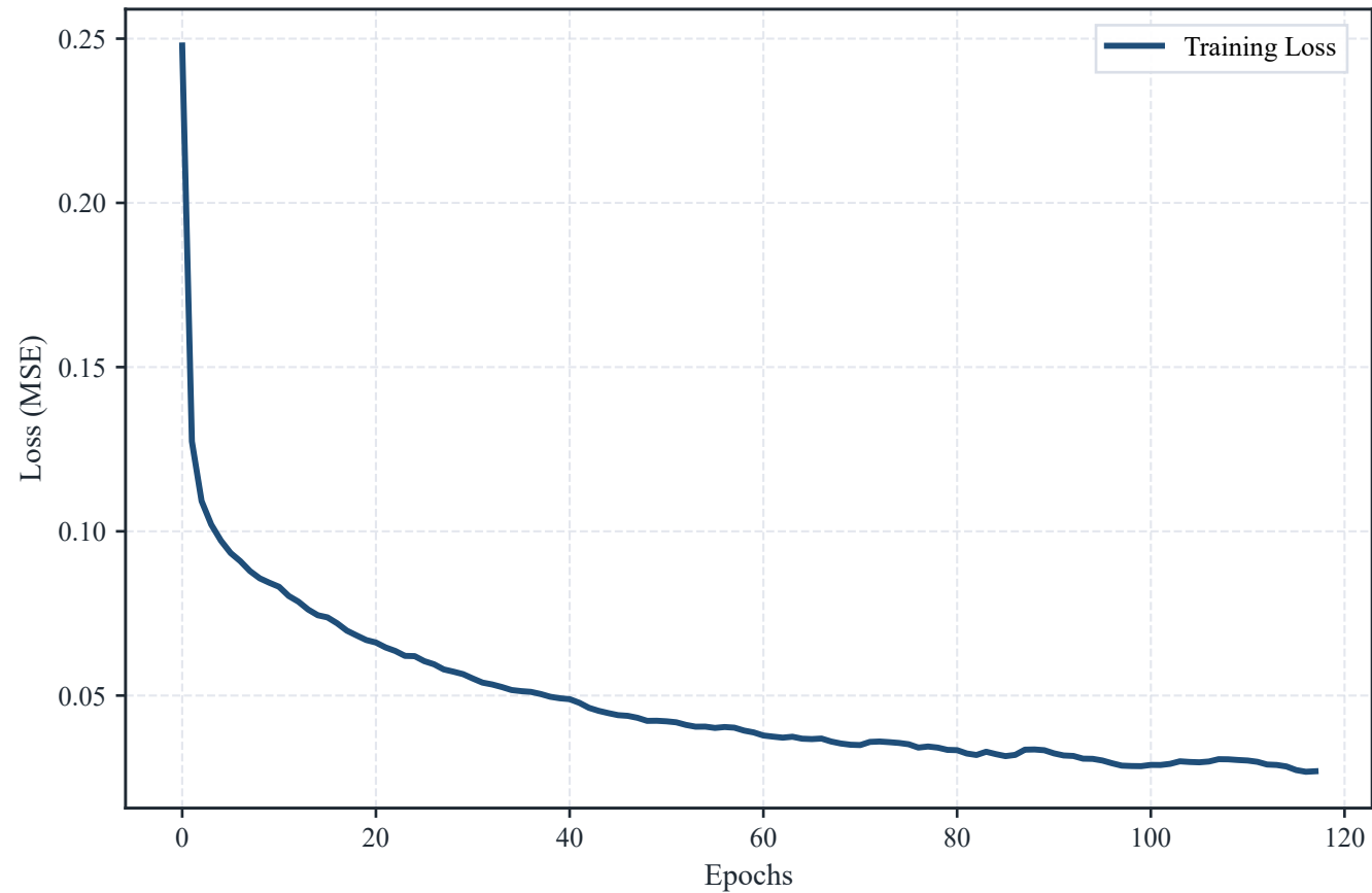
Training Loss Convergence (Optimized)
