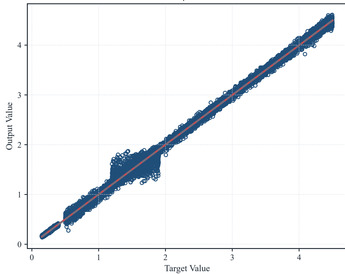
Test Set | R=0.9990
