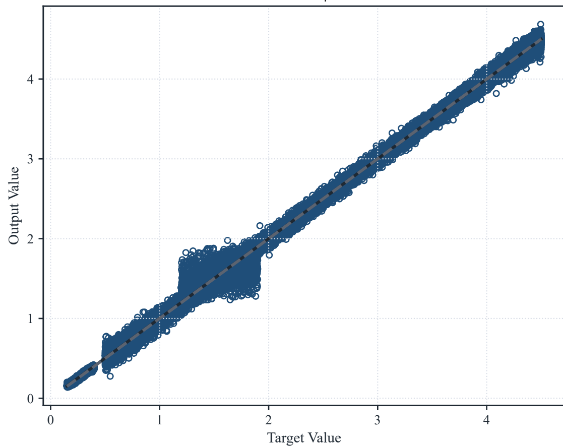
Overall Dataset | R=0.9995
