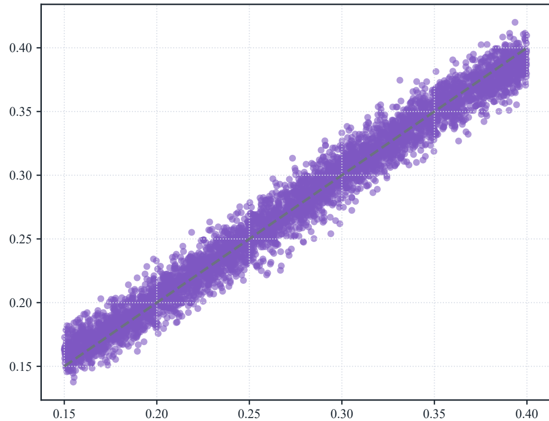
Radius Accuracy (RMSE: 1.14 cm)
