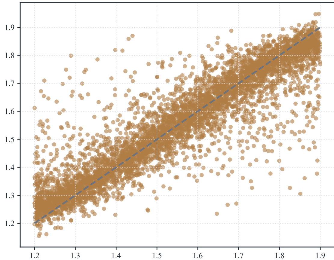
Height Accuracy (RMSE: 8.44 cm)
