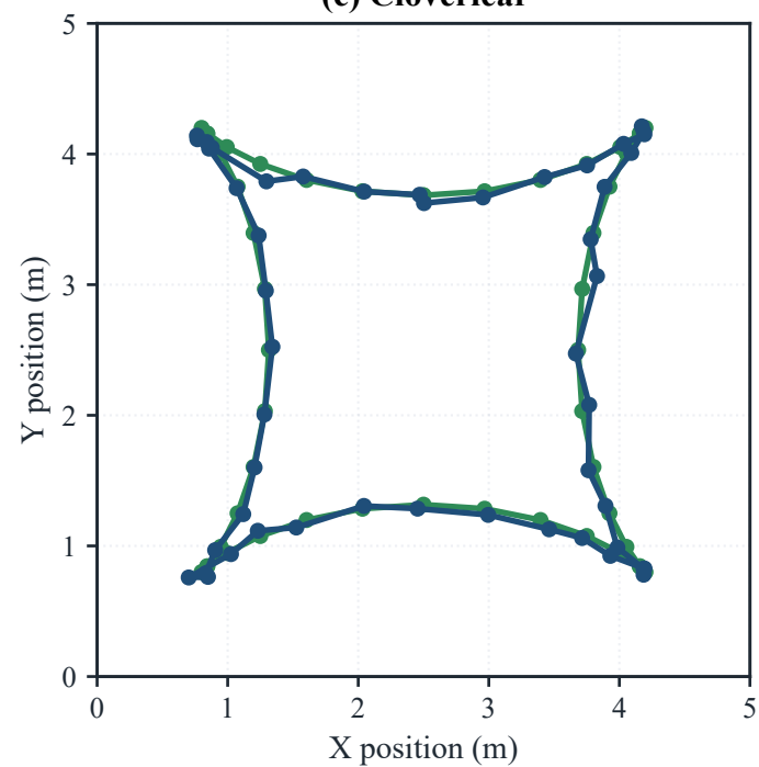
(c) Cloverleaf
