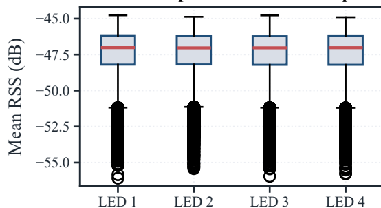
Mean RSS per LED Across Samples
