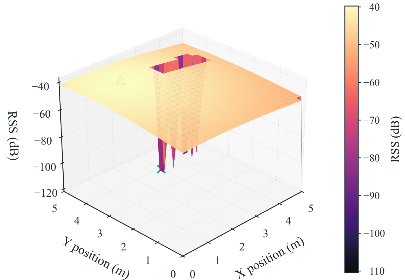
LED 4 RSS Surface
