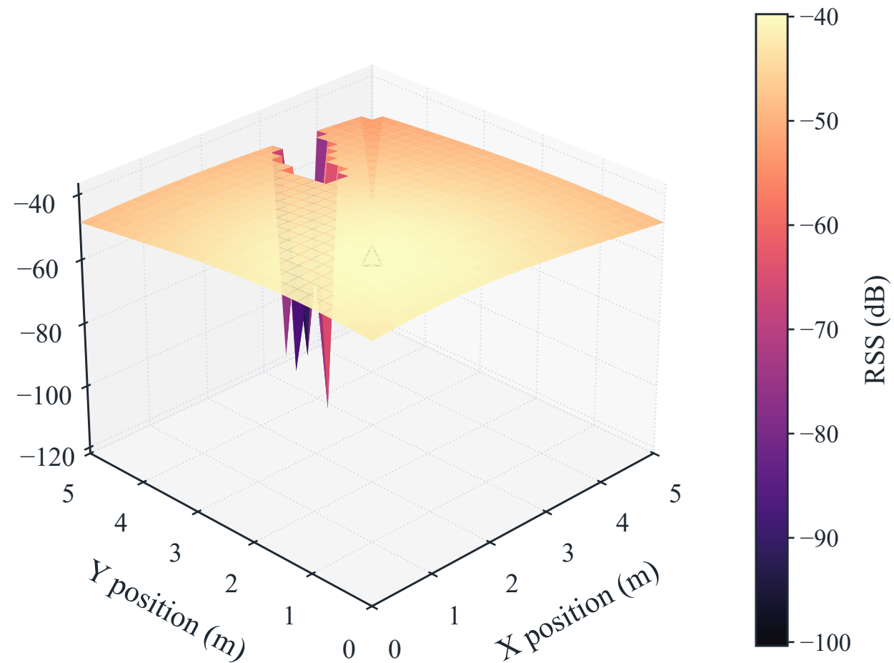
LED 3 RSS Surface
