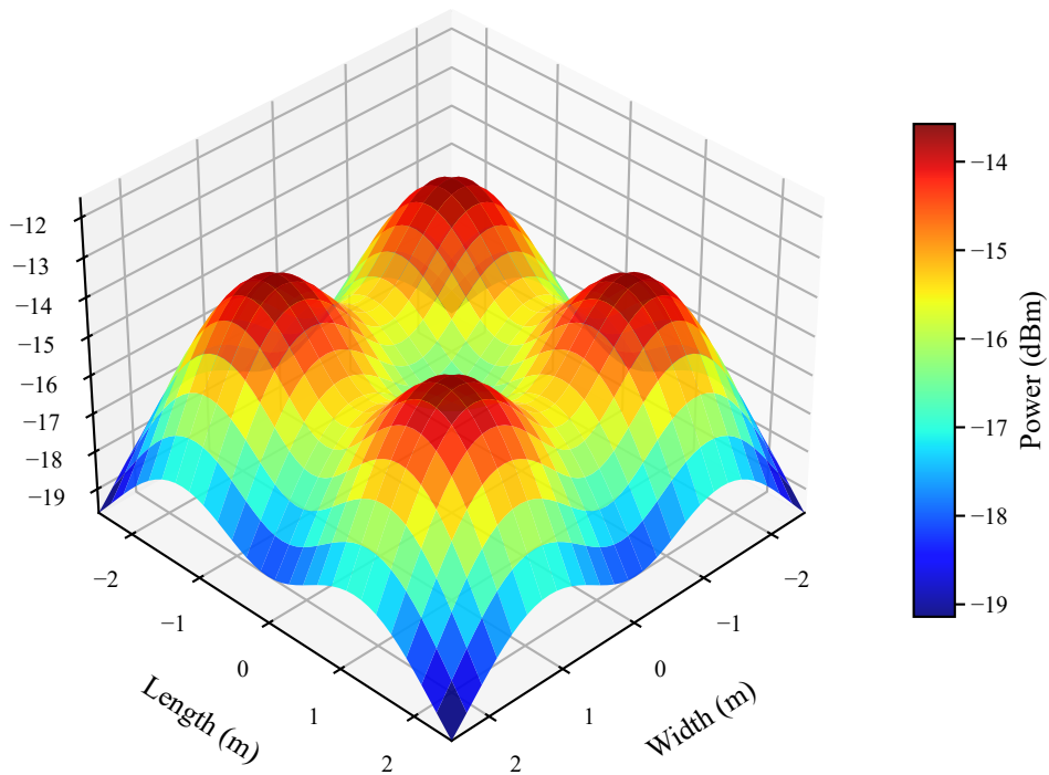
Simulation Received Power Profile
