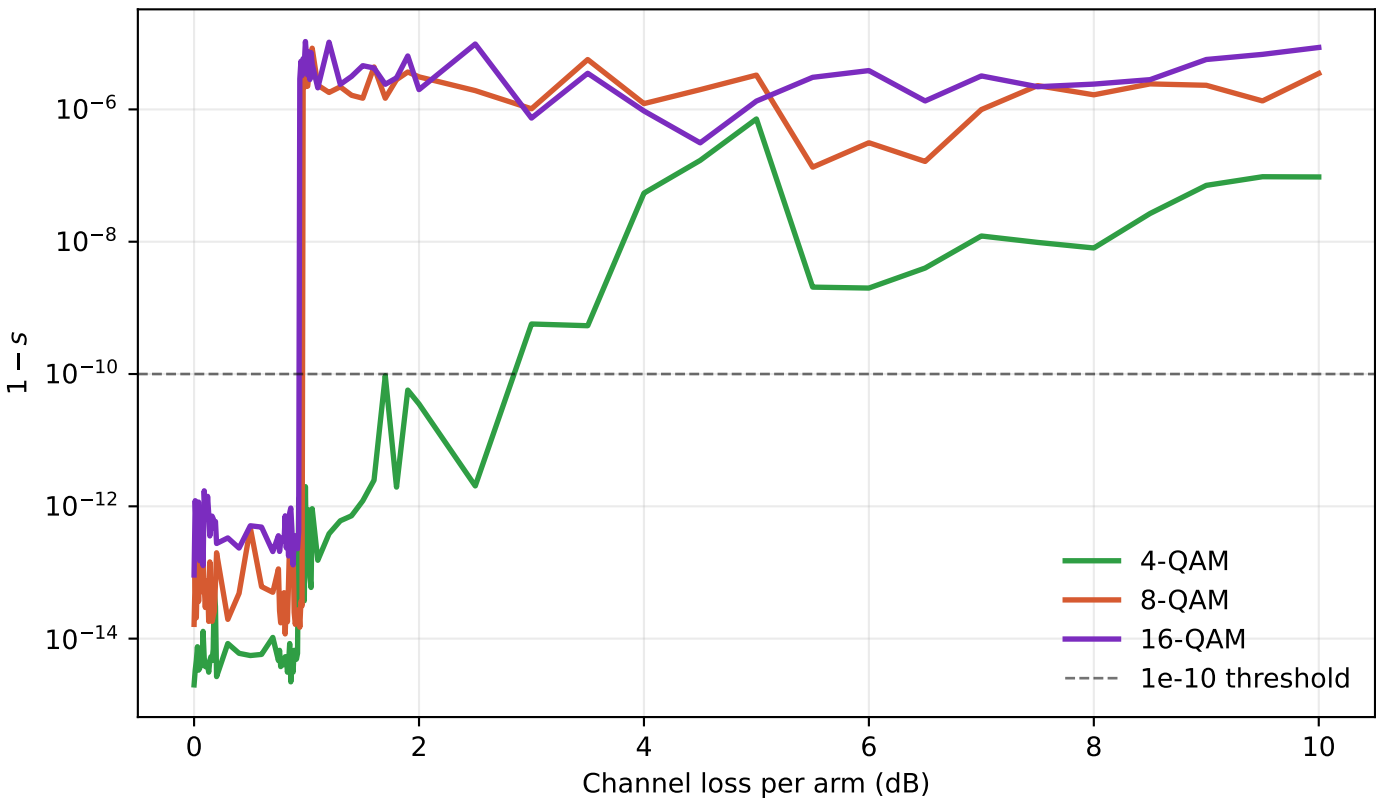
Deviation of POVM scale from 1
