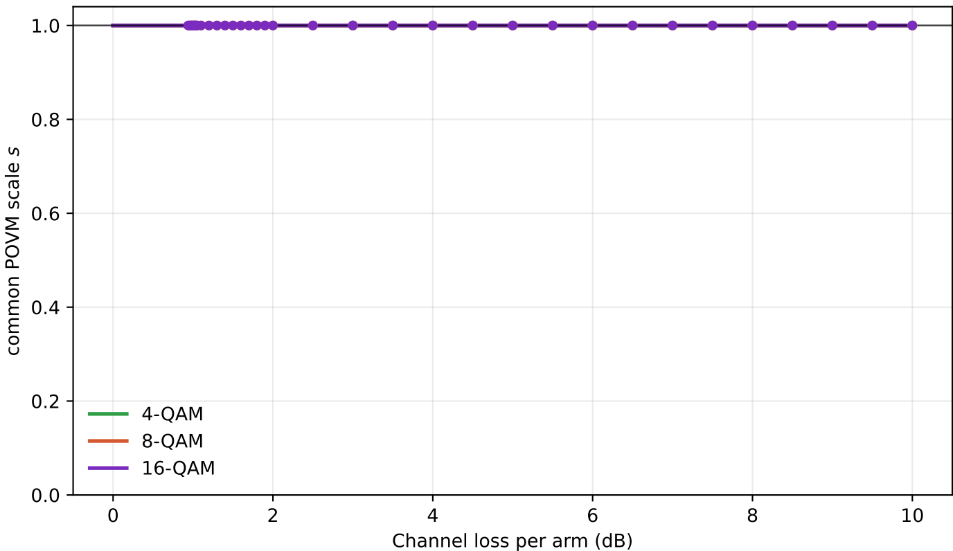
Full-state/raw-label SRM POVM scale at optimized d
