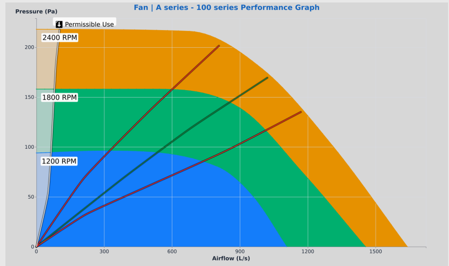
Fan | A series - 100 series Performance Graph
