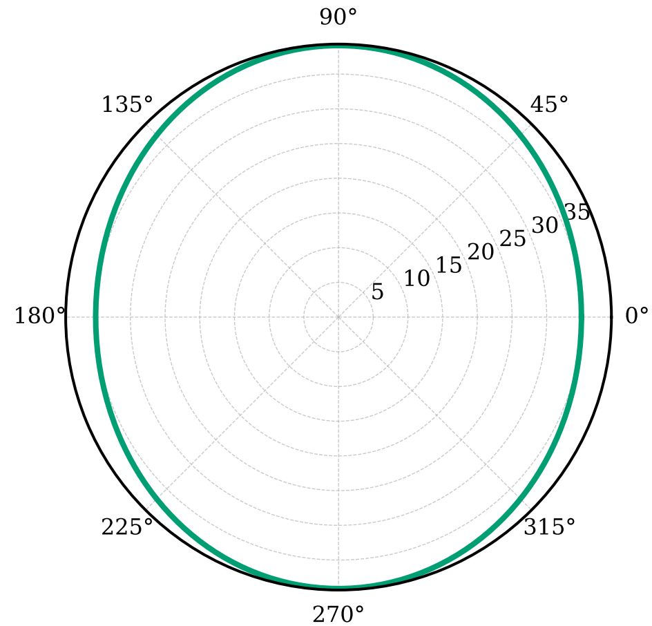
XY Plane
