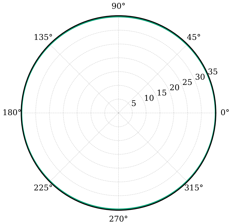
ZX Plane
