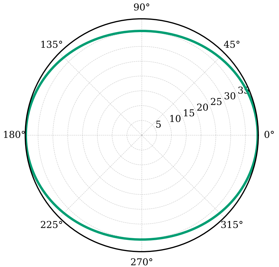
YZ Plane
