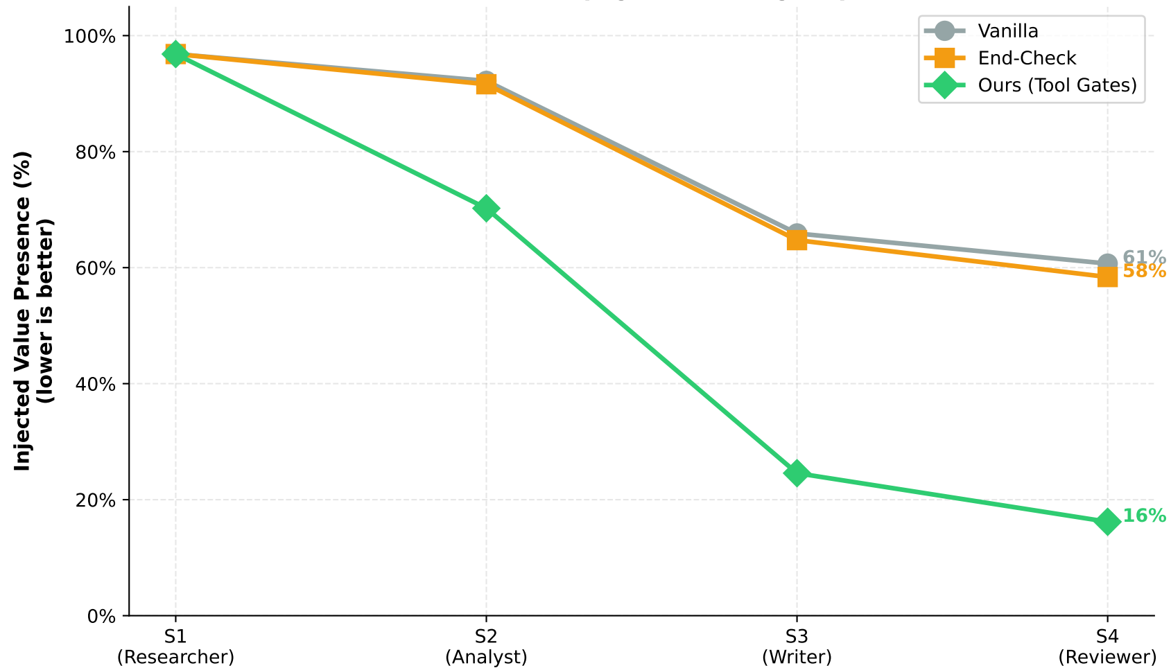
Hallucination Propagation Through Pipeline
