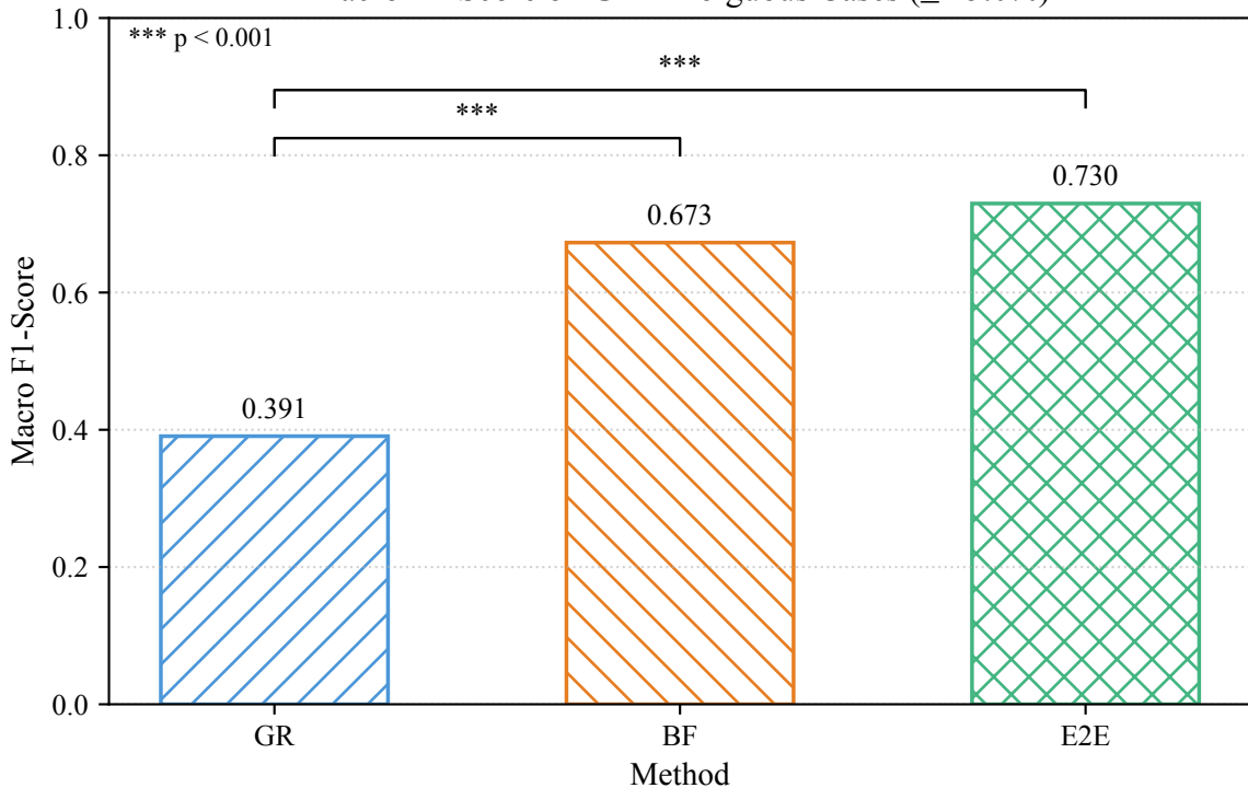
Macro F1-Score on GR Ambiguous Cases ( \leq 25.0\% )
