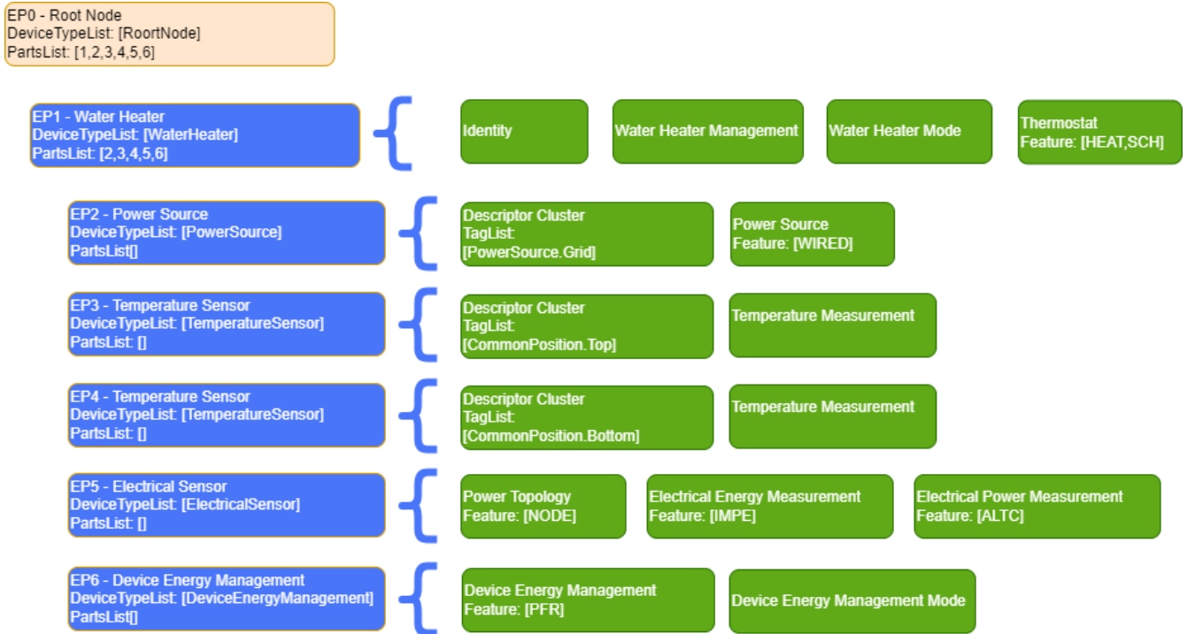
Figure 17. Example of a Water Heater
