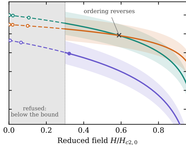
(b) at 4.2 K
