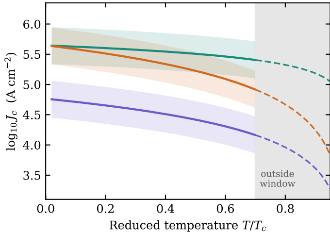
(a) at H/H_{c2,0} = 0.5
