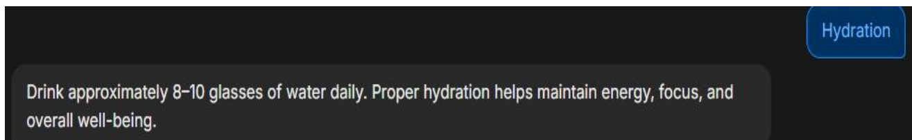
Figure 6: Hydration Interaction
