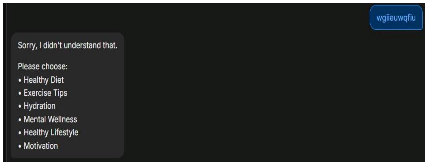
Figure 9: Fallback Response
