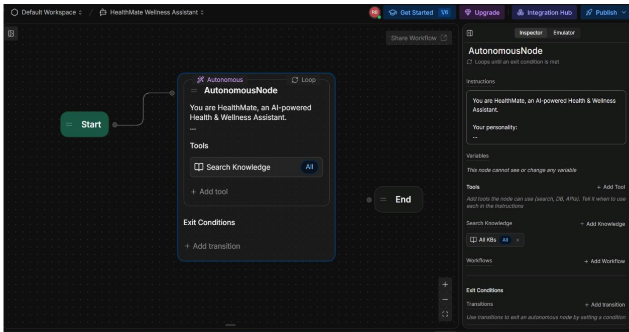
Figure 2: Workflow Design
