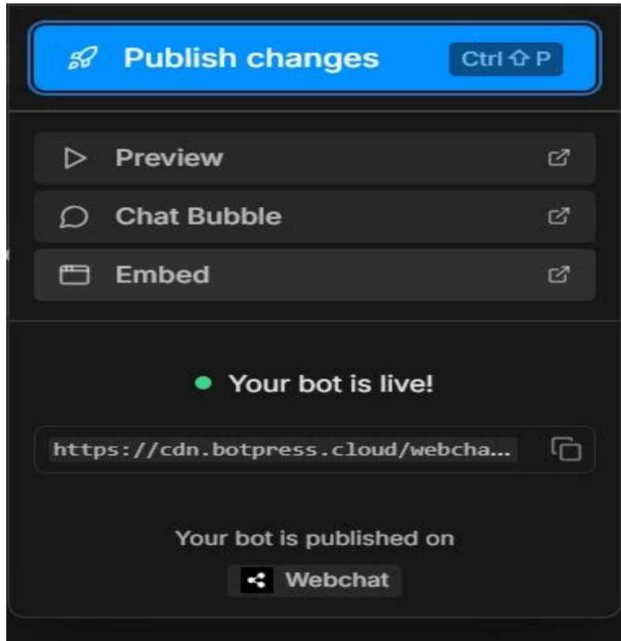
Figure 10: Published Chatbot
