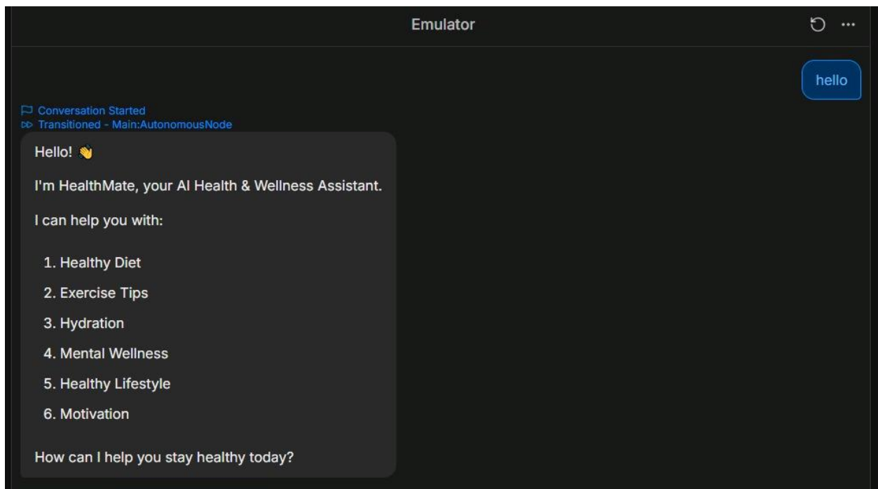
Figure 3: Welcome Message
