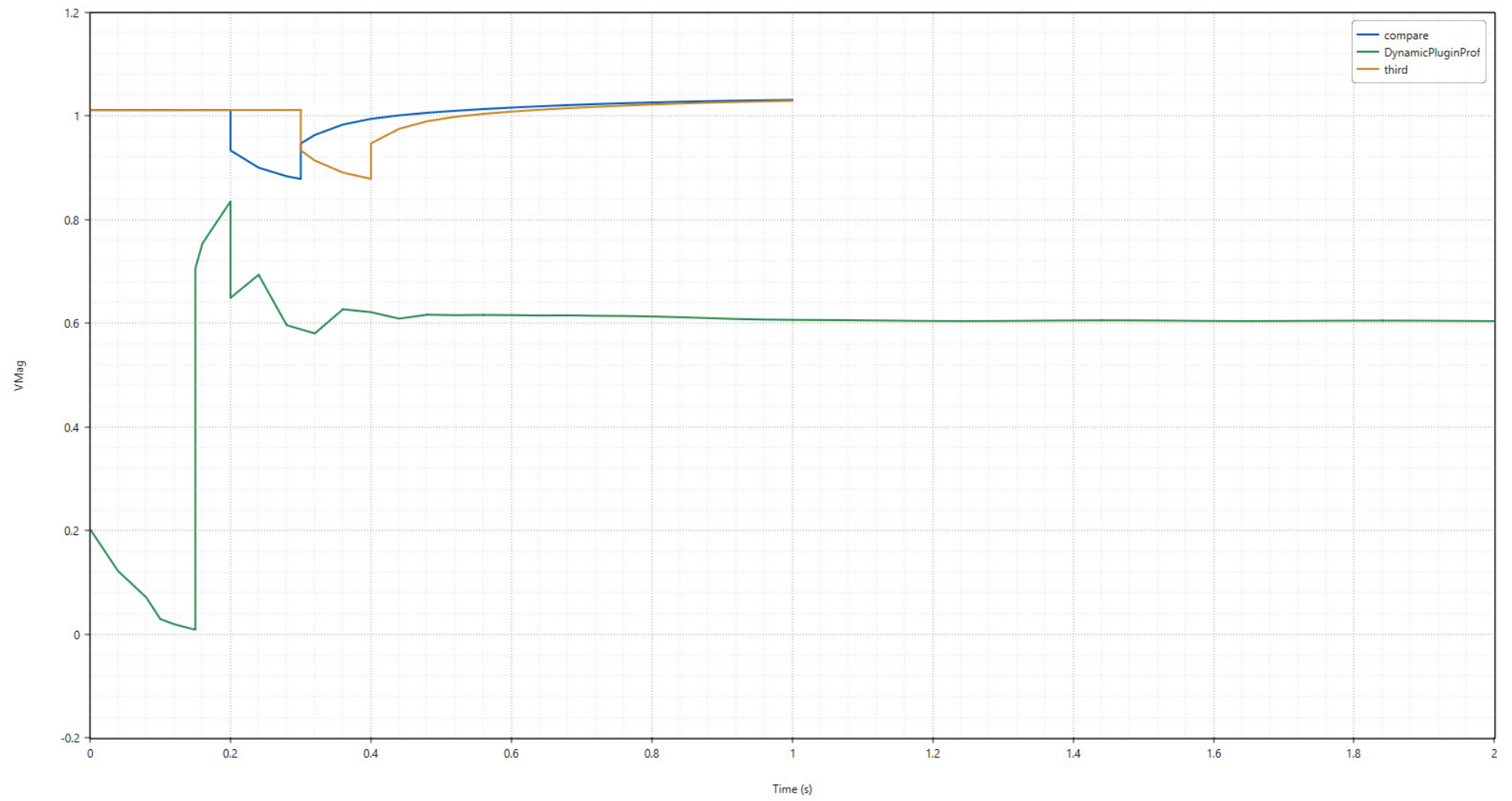
Busbars [3] - Voltage (PU)
